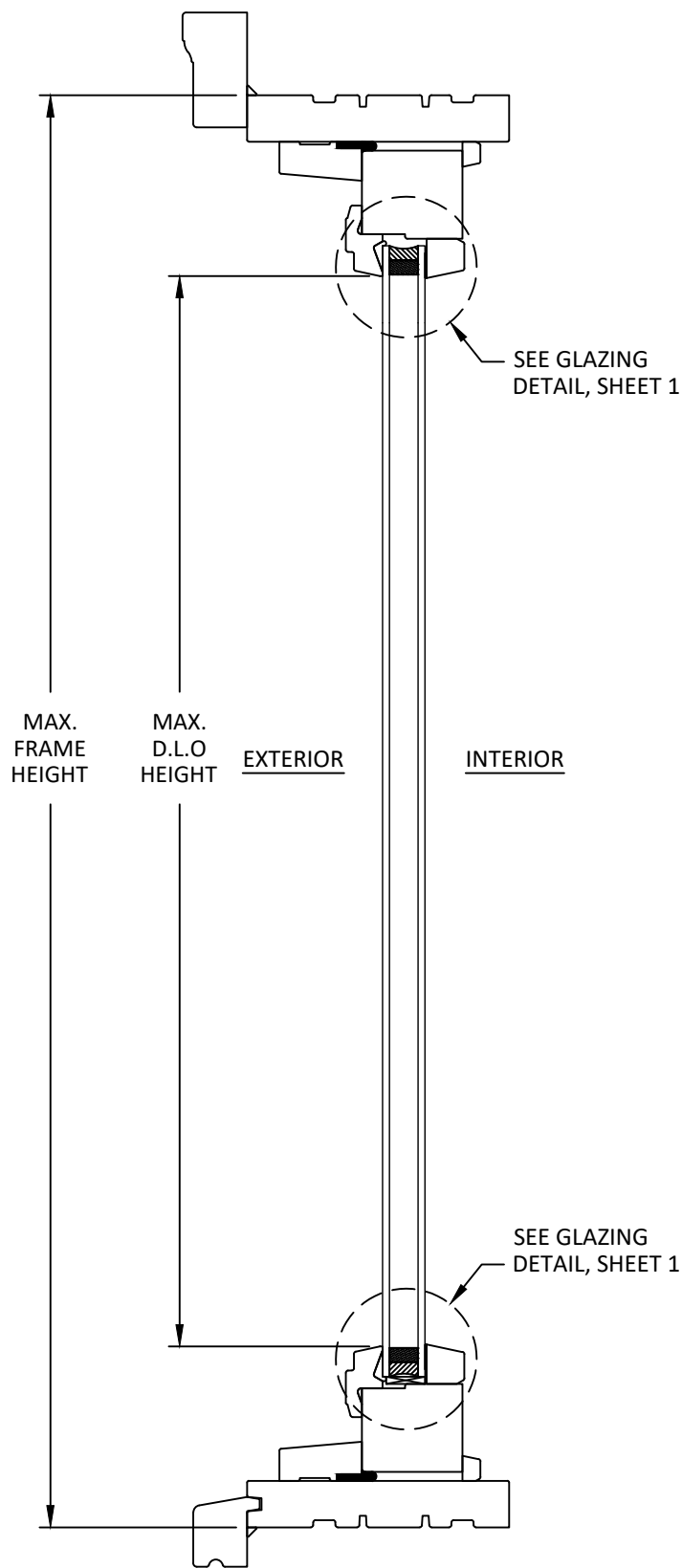
VERTICAL SECTION 4-9/16" FRAME RECTANGULAR
