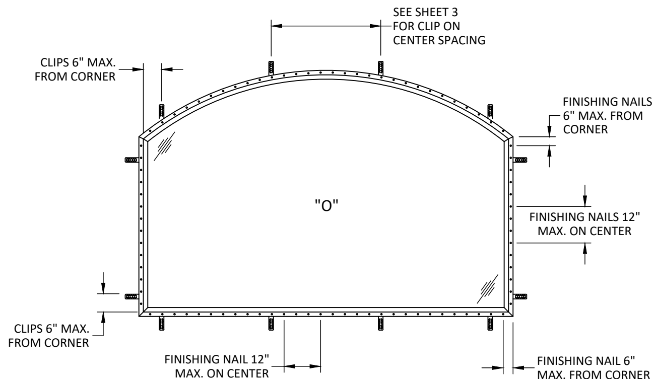
ANCHOR LAYOUT ARCHTOP
