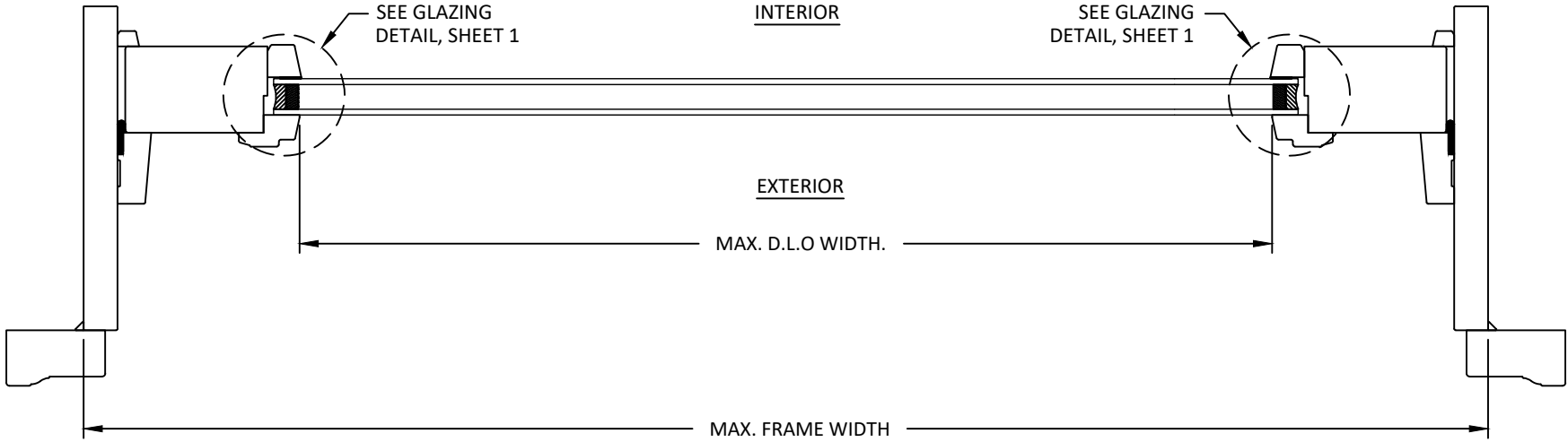
C 7 HORIZONTAL SECTION 6-9/16" FRAME SPRINGLINE
