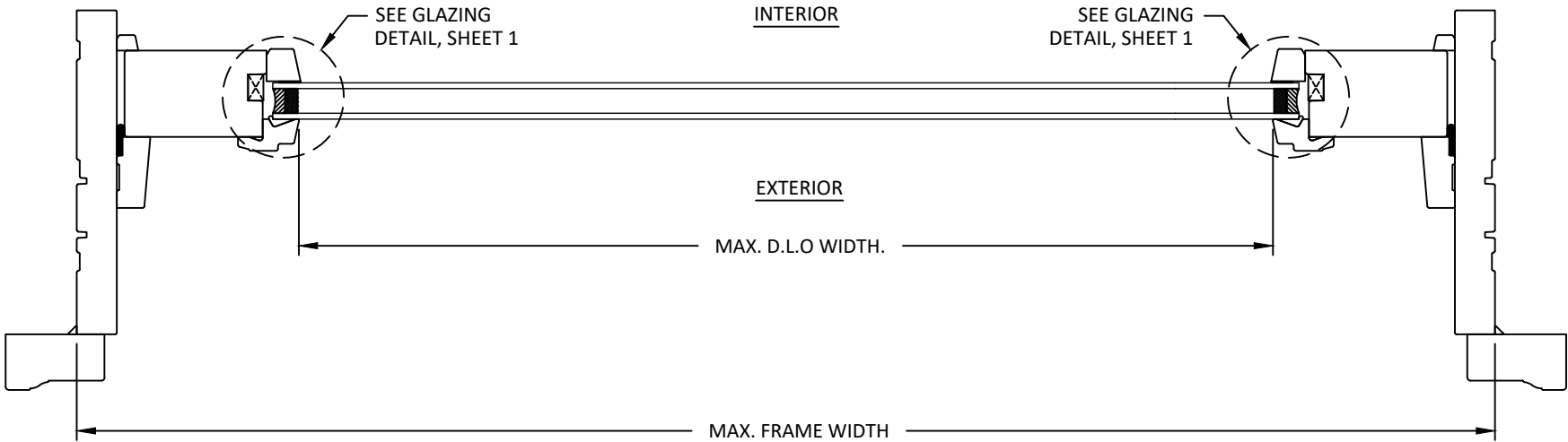
A 7 HORIZONTAL SECTION 6-9/16" FRAME RECTANGULAR
