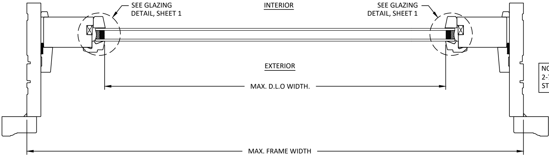
B 7 HORIZONTAL SECTION 6-9/16" FRAME ARCHTOP
