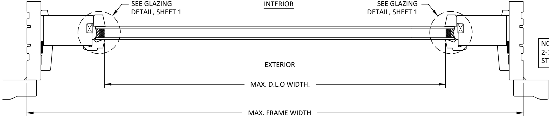
B 6 HORIZONTAL SECTION 4-9/16" FRAME ARCHTOP
