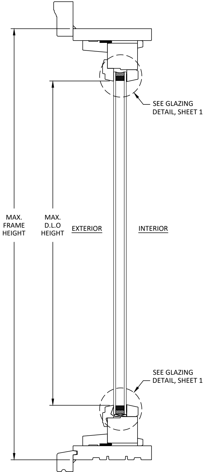
VERTICAL SECTION 4-9/16" FRAME ARCHTOP
