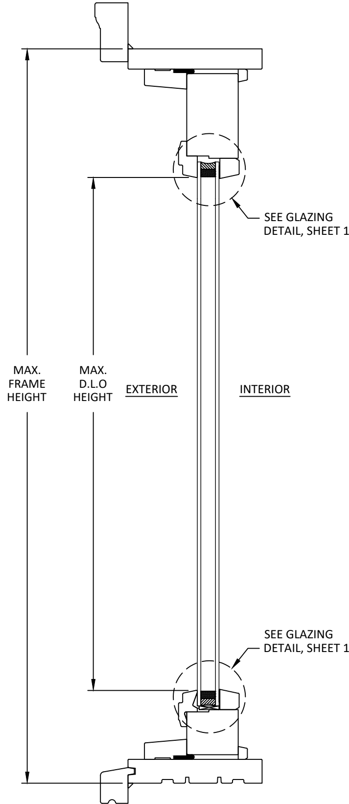
VERTICAL SECTION 4-9/16" FRAME SPRINGLINE
