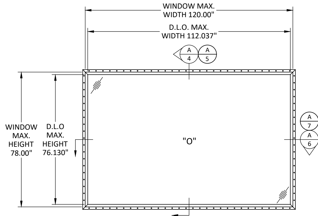
ELEVATION RECTANGULAR
