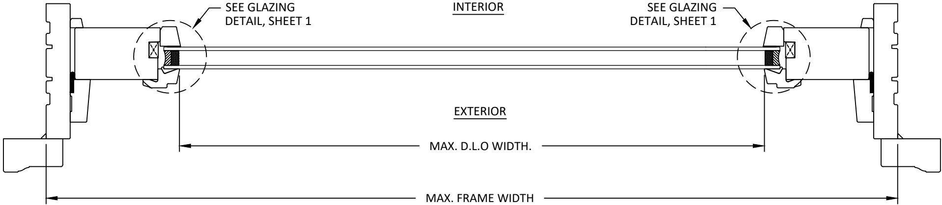
A 6 HORIZONTAL SECTION 4-9/16" FRAME RECTANGULAR
