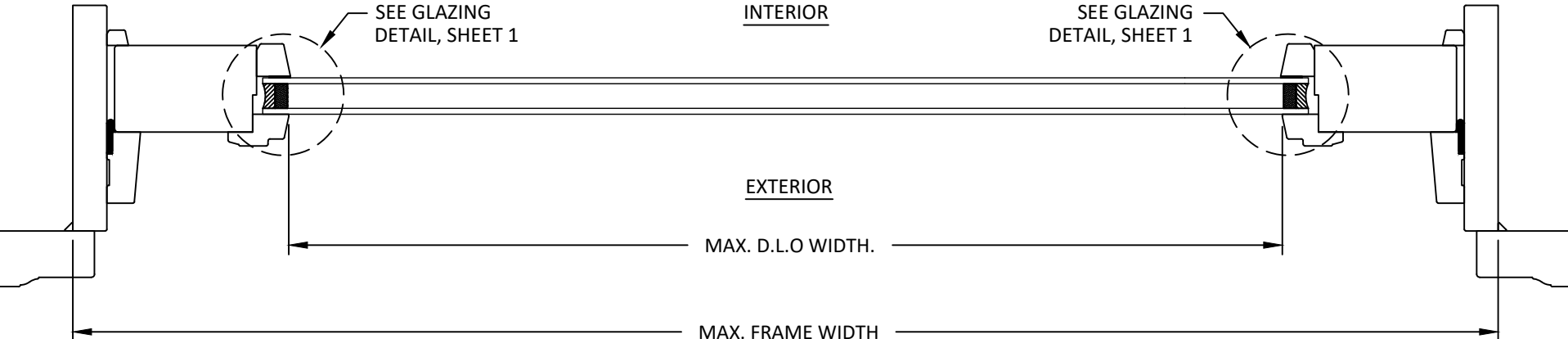
C 6 HORIZONTAL SECTION 4-9/16" FRAME SPRINGLINE
