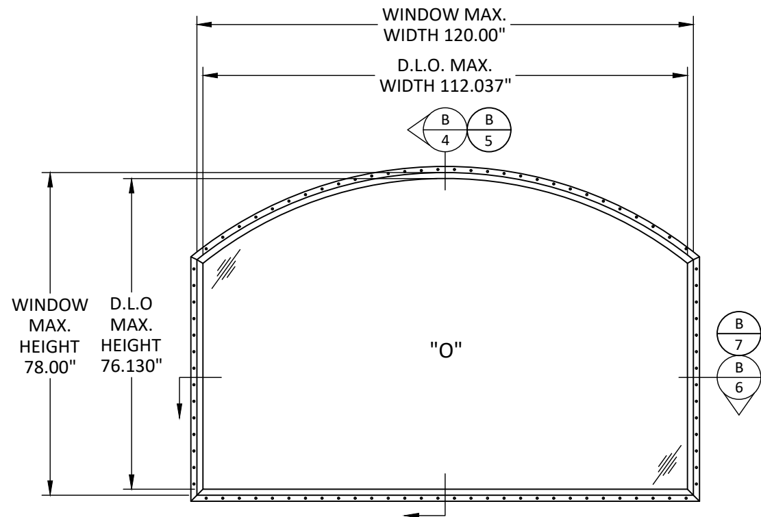
ELEVATION ARCHTOP
