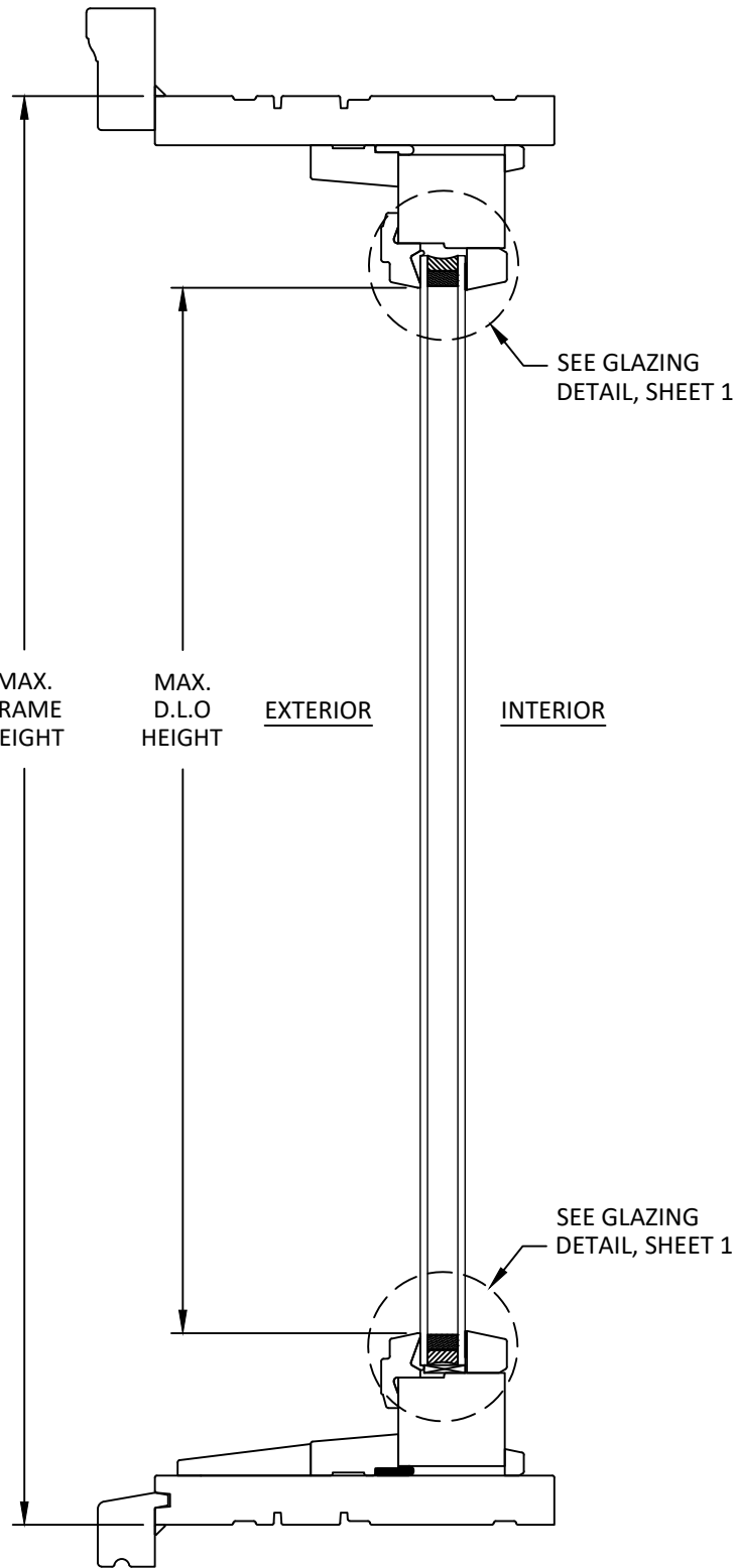
A 5 VERTICAL SECTION 6-9/16" FRAME RECTANGULAR
